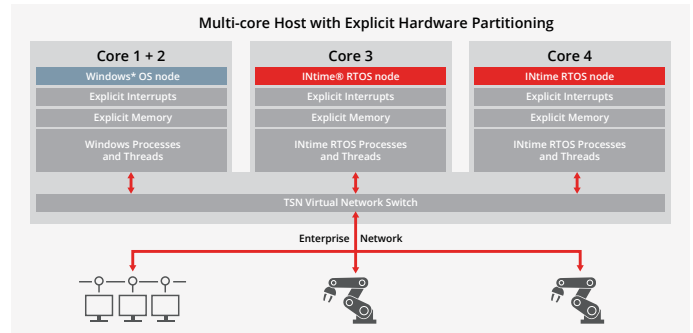
Depicted here is an example of embedded virtualization at work in an explicitly partitioned system that dedicates two cores each with their own processor core, memory, and I/O resources to time-critical control tasks and an additional two cores to non-time-critical network, database, and user interface functions.
