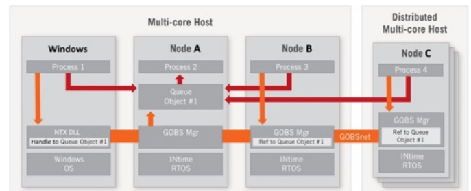
The red arrows in the figure above represent a shared inbound queue for Node A. The orange arrows between the A, B, and Windows Nodes represent references to the handle of Object #1 by different global objects (GOBS) Managers on each node. The GOBSnet bar located between Nodes B and C represents the same handle referencing function as the other orange lines, with the principal difference that the communication request is being made by a distributed host located elsewhere on the network.
